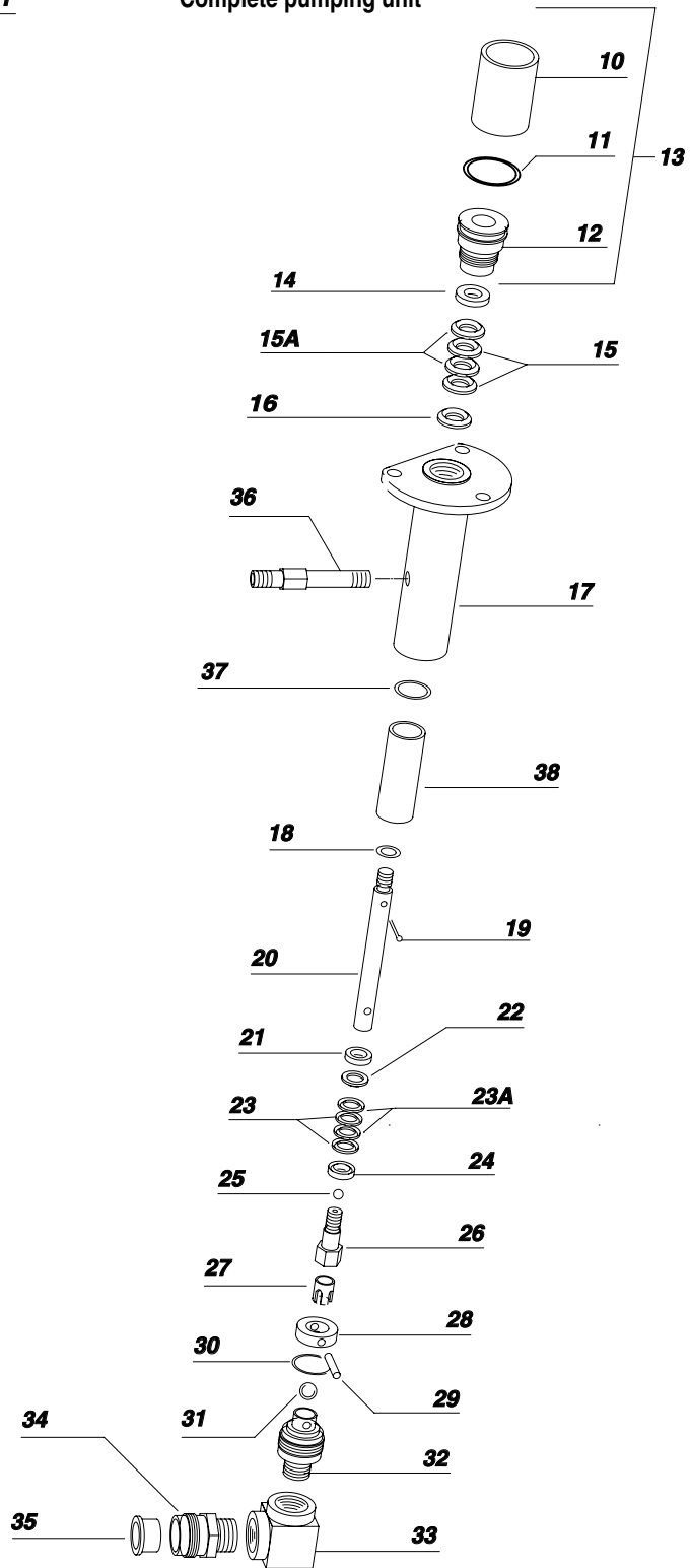
Complete pumping unit
