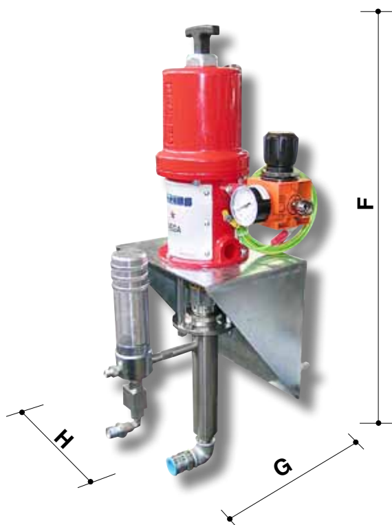
WALL BRACKET Version
